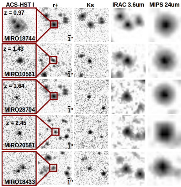
Fig. 2. From left to right: ACS-HST I, r+ Subaru, Ks COSMOS, IRAC 3.6 \mu\text{m} , MIPS 24 \mu\text{m} band cutouts of the five MIRO targets. The target name, position, cutouts scale, and redshift derived from the SINFONI data are also labelled. For display purposes, 3'' \times 3'' ACS-HST cutouts show the regions in the red boxes superimposed on the r+ cutouts.
