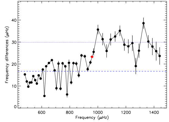
Fig. A.15. Consecutive frequency differences (KIC 11717120); that is, the separations between the fitted peaks for NAvPSD. Two levels are shown: one around \Delta\nu/2 , corresponding to p -modes (blue dashed line with a weighted mean of 16.71 \pm 0.09 \mu\text{Hz} ), and other around \Delta\nu , corresponding to pseudo-modes (blue dotted line with a weighted mean of 29.85 \pm 0.66 \mu\text{Hz} ). The red symbol is the estimation of the acoustic cut-off frequency ( 958.38 \pm 11.56 \mu\text{Hz} ).
