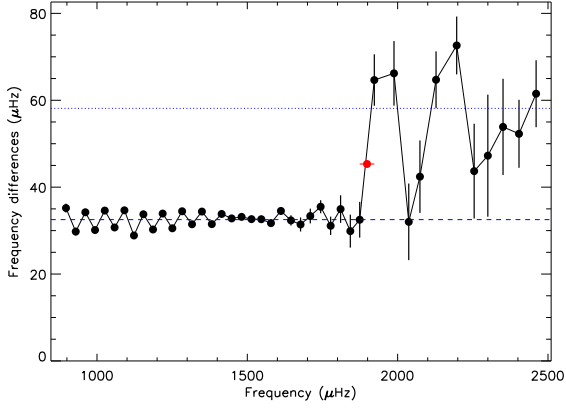
Fig. A.9. Consecutive frequency differences (KIC 9812850); that is, the separations between the fitted peaks for NAvPSD. Two levels are shown: one around \Delta\nu/2 , corresponding to p -modes (blue dashed line with a weighted mean of 32.53 \pm 0.12 \mu\text{Hz} ), and other around \Delta\nu , corresponding to pseudo-modes (blue dotted line with a weighted mean of 58.13 \pm 2.39 \mu\text{Hz} ). The red symbol is the estimate of the acoustic cut-off frequency ( 1898.08 \pm 24.29 \mu\text{Hz} ).
