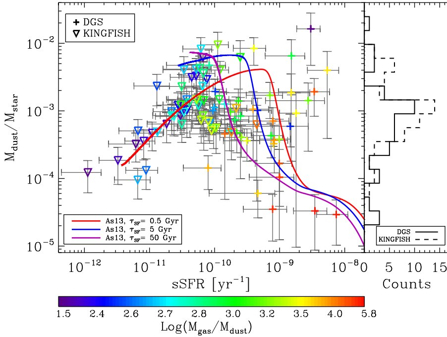
Fig. 11. Dust-to-stellar mass ratios for the DGS (crosses) and KINGFISH (downwards triangles) samples as a function of sSFR, colour coded by the gas-to-dust mass ratio (G/D), M_{\text{gas}}/M_{\text{dust}} , from Rémy-Ruyer et al. (2014). The distribution of M_{\text{dust}}/M_{\text{star}} is indicated on the side for both samples: solid line for DGS and dashed line for KINGFISH. Modelled evolutionary tracks from Asano et al. (2013) are shown, for different star formation timescales ( \tau_{\text{SF}} = 0.5, 5 and 50 Gyr), with the red, blue, and purple lines.
