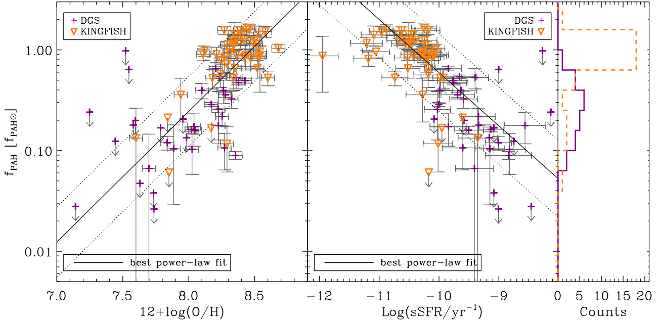
Fig. 7. The PAH mass fractions for the DGS (purple crosses) and KINGFISH (orange downward triangles) samples as a function of metallicity (left panel) and sSFR (right panel). The parameter f_{\text{PAH}} is expressed in units of f_{\text{PAH}\odot} , with f_{\text{PAH}\odot} = 4.57\% . The distribution of f_{\text{PAH}} is indicated on the side for both samples: plain purple line for DGS galaxies and dashed orange line for the KINGFISH sample. In each panel, the best power-law fit is indicated as a solid line, together with the 1\sigma dispersion as dotted lines.
