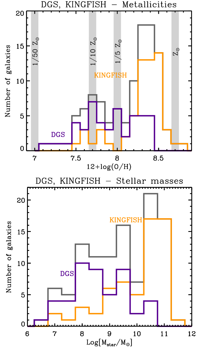
Fig. 1. Metallicity (top), and stellar mass (bottom) distributions of the DGS (purple), KINGFISH (orange) samples. The total distribution is indicated in grey. In the top panel, solar metallicity is indicated here to guide the eye, as well as the 1/50 , 1/10 , and 1/5 Z_{\odot} values.
