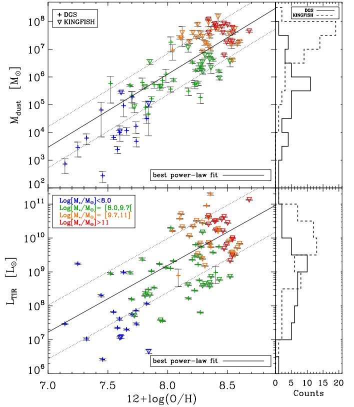
Fig. 6. Dust masses (top), TIR luminosities (bottom) for the DGS (crosses), and KINGFISH (downward triangles) samples as a function of metallicity, colour coded with M_{\text{star}} . The best power-law fit is indicated with a black line, and the 1\sigma dispersion is indicated with dotted lines for the two panels. The distribution of each parameter is indicated on the side of each panel for both samples: solid line for DGS and dashed line for KINGFISH.
