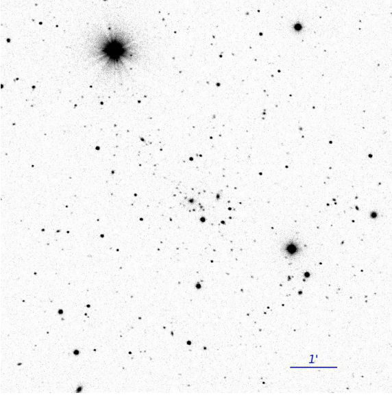
Fig. 9. PSZ1 G048.22-65.03 RTT150 i' -band image. This cluster is too distant to be identified with DSS ( z \approx 0.42 ) and there are no SDSS data in this field.
