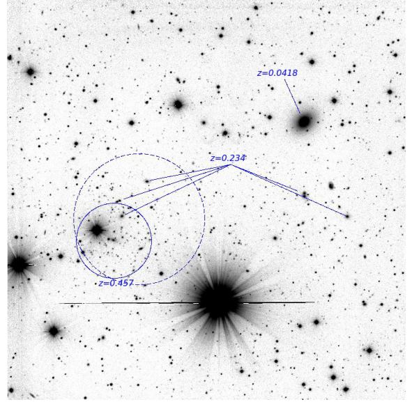
Fig. 15. PSZ1 G109.14-28.02 RTT150 i' -band image, dashed circle ( 2' radius) shows the location of Planck SZ source. In addition to the rich cluster at z = 0.457 (solid circle), there are also two galaxy groups at z = 0.234 , a nearby elliptical galaxy at z = 0.0418 , and a bright star in the field.
