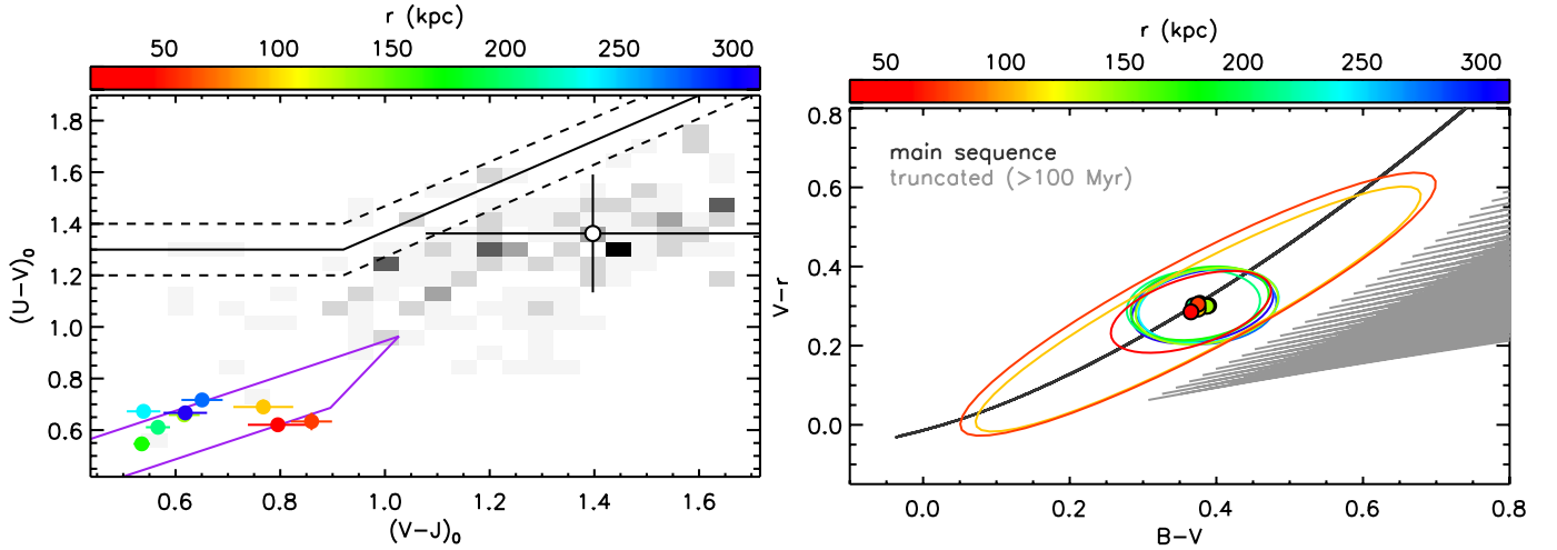
Fig. 10. Left: median rest-frame U-V and V-J colors, derived from SED modeling, of star-forming satellites (filled circles, colored as a function of distance to the central) and centrals (open circle and gray density histogram). The purple lines show the expected colors of stellar populations models of varying age following a “main-sequence” SFH, assuming E(B-V) < 0.3 . Right: median observed B-V and V-r colors of satellites, as a function of distance to the central, compared to the expected colors of a star-forming model (main-sequence SFH, black) and a constant SFR one observed \geq 100 Myr after the quenching of star formation (gray). We here include dust extinction with E(B-V) = 0-2 . The ellipses show the dispersion of B-V and V-r values in each radial bin.
