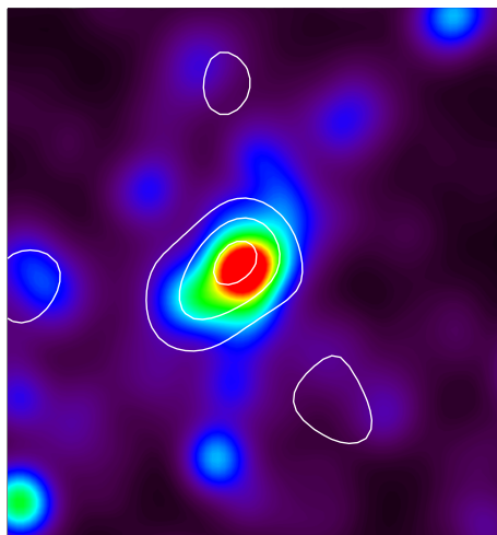
Fig. A.2. Same as Fig. A.1, for MS 0451.6-0305.
