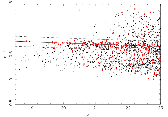
Fig. 3. Colour–magnitude diagram in the field of MS 1621.5+2640. The black points are the galaxies located at r < 500'' from the cluster centre. The red dots are galaxies with r < 200'' and a z_{\text{phot}} compatible with the cluster redshift. The straight line is the best fit to the red sequence and the dashed lines are the 3\sigma limits of the red sequence. At the cluster redshift ( z = 0.43 ), the expected colour, computed with the synthetic evolutionary code of Bruzual & Charlot (2003), is r' - i' = 0.77 .
