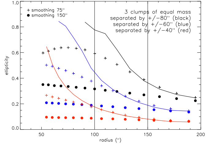
Fig. 5. Ellipticity of simulated clusters formed by 3 mass clumps with NFW profile, and smoothed with 2 different kernels. The continuum line is the ellipticity measured on the unsmoothed data. For comparison the ellipticity of the observed clusters was measured in radii ranging from 100 to 150'' approximately.
