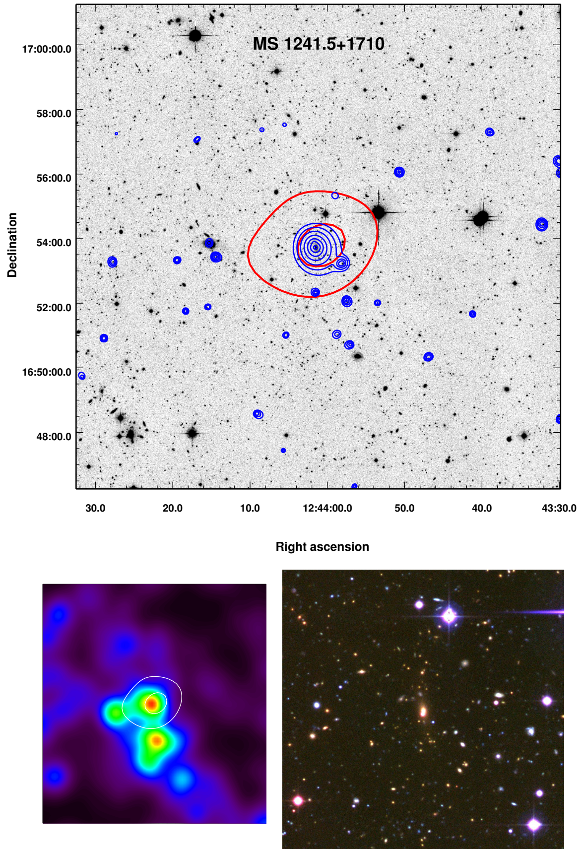
Fig. A.8. Same as Fig. A.1, for MS 1241.5+1710.
