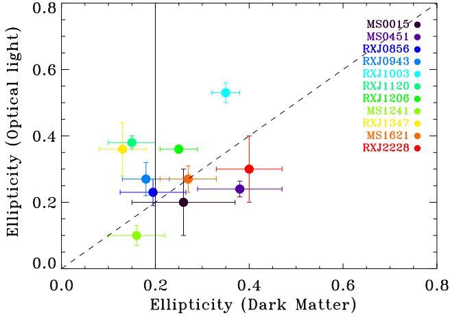
Fig. 6. Ellipticity of the optical light distribution versus the ellipticity of the dark matter. The vertical line separates the cluster sample between the circular clusters with \epsilon < 0.2 and the elliptical or irregular clusters.
