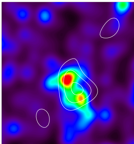
Fig. A.5. Same as Fig. A.1, for RXC J1003.0+3254.
