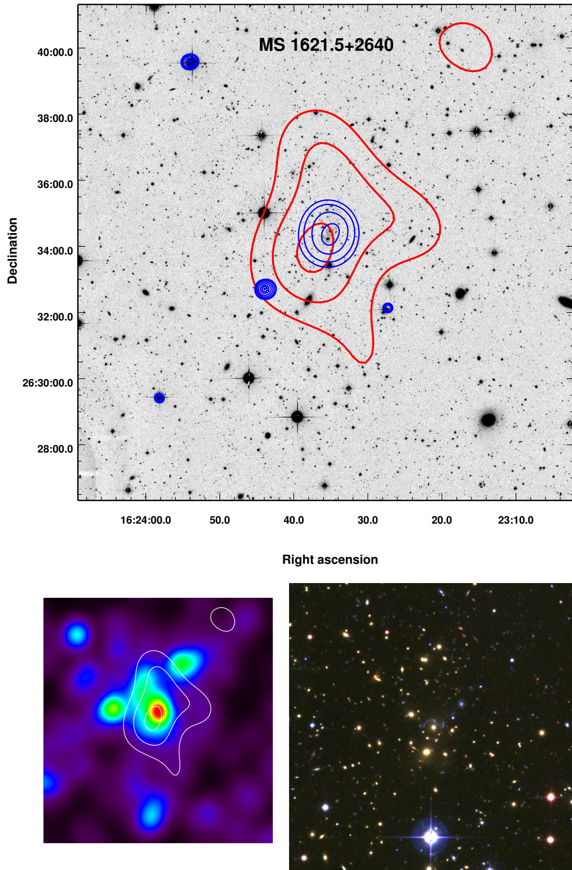
Fig. A.10. Same as Fig. A.1, for MS 1621.5+2640.
