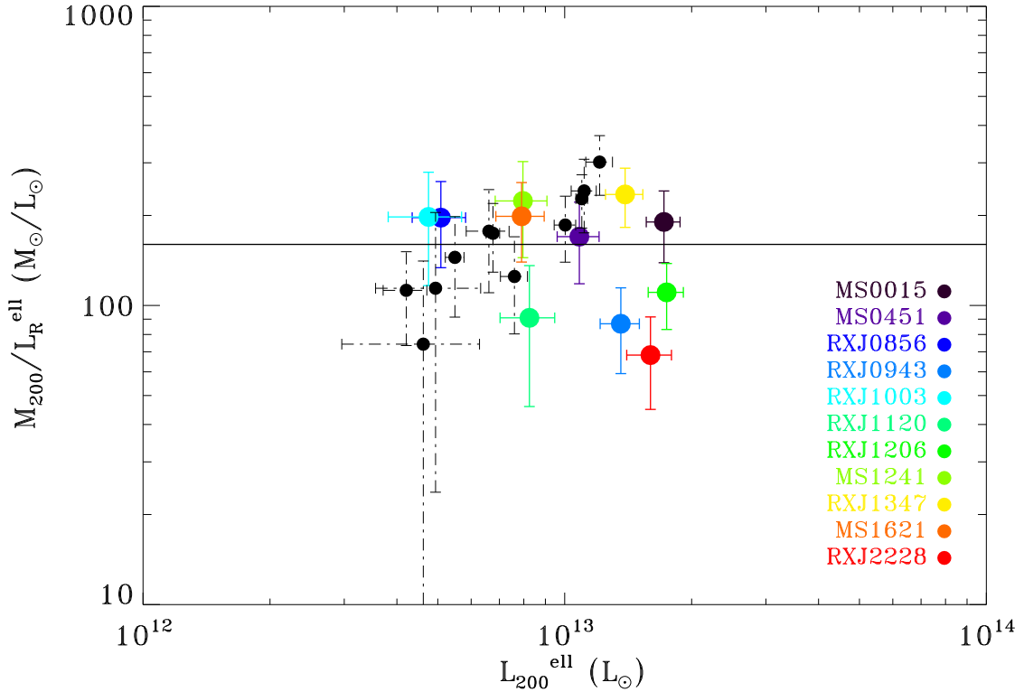
Fig. 9. Mass-to-light ratio versus the total luminosity L_{200}^{2D} for the 11 clusters of the sample (colour points) and the 11 clusters added from the sample of Bardeau et al. (2007). The average value M/L = 166 in solar units is drawn as a solid line.
