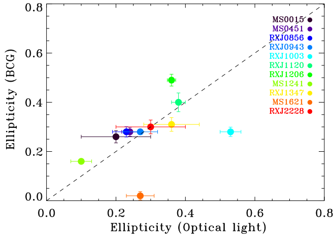
Fig. 4. Ellipticity of the global light distribution of the clusters versus the ellipticity of the brightest central galaxy.
