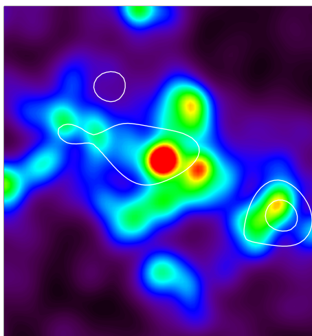
Fig. A.11. Same as Fig. A.1, for RX J2228.5+2036.
