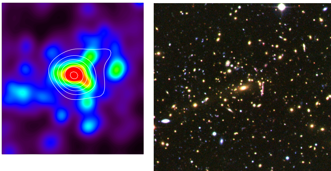
Fig. A.7. Same as Fig. A.1, for RXC J1206.2-0848.
