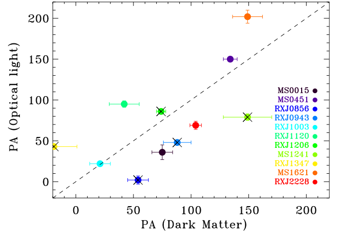
Fig. 7. Orientation of the optical light distribution versus the dark matter. The circular clusters with an ellipticity \epsilon < 0.2 are marked with a cross.
