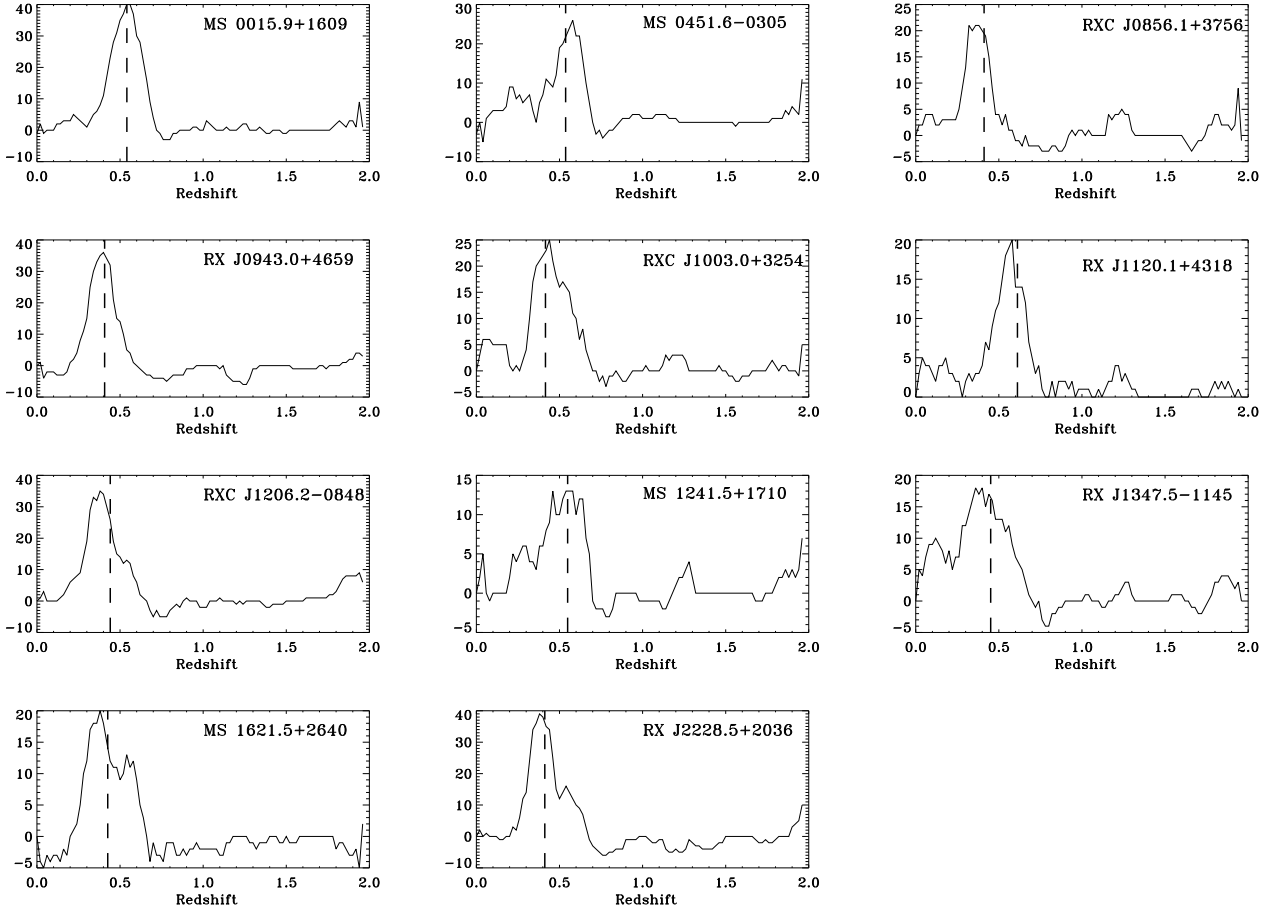
Fig. 2. Over-densities in the photometric redshift distribution for each cluster. In each panel the vertical line shows the spectroscopic redshift of the cluster. The plot represents the redshift distribution of the central area defined as R < 5' minus the distribution of an annulus of same area starting at R = 10' .
