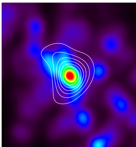
Fig. A.9. Same as Fig. A.1, for RX J1347.5-1145.
