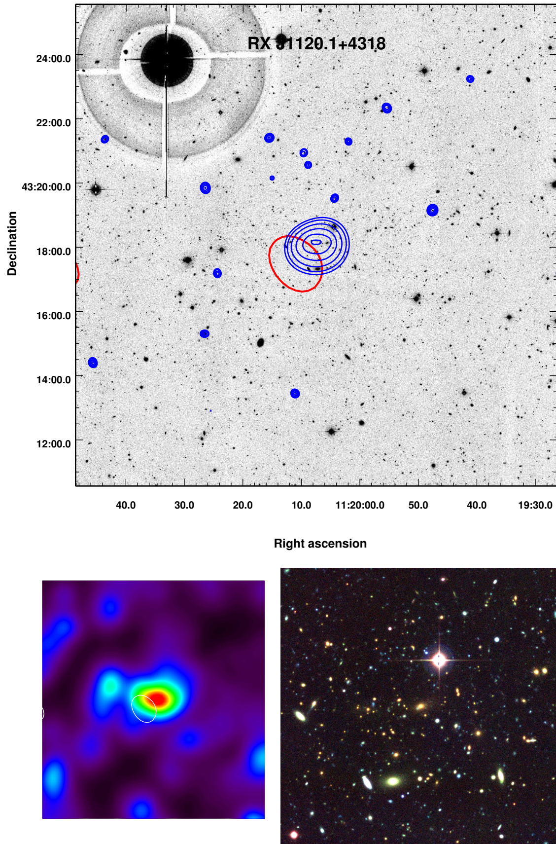
Fig. A.6. Same as Fig. A.1, for RX J1120.1+4318.
