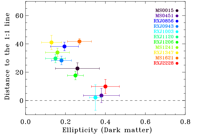
Fig. 8. Orthogonal deviation (in degrees) from the 1:1 line for the dark matter orientation (PA(DM)) compared to the light distribution orientation (PA(light)) versus the ellipticity of the dark matter distribution. The more elliptical this distribution, the better the alignment between light and dark matter.
