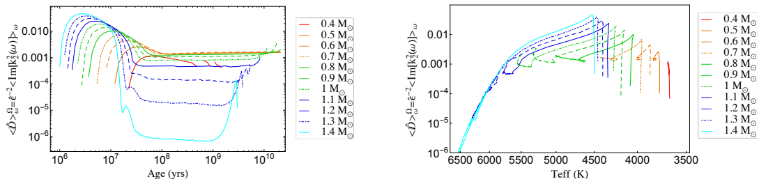
Fig. 4. Evolution of the frequency-averaged tidal dissipation at fixed normalized angular velocity, \langle \mathcal{D} \rangle_\omega^{\Omega} = \epsilon^{-2} \langle \text{Im} [k_2^2(\omega)] \rangle_\omega , as a function of time (left panel) and effective temperature (right panel) for stellar masses ( M_s ) from 0.4 to 1.4 M_\odot (the colours are the same as in Fig. 2).
