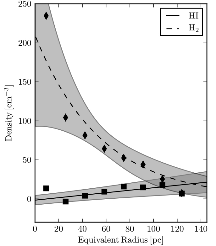
Fig. 14. Density of H I and H 2 as a function of the distance toward the center of W43 (equivalent radius). The diamonds and the dashed line represent the molecular hydrogen, whereas squares and the solid line represent the atomic hydrogen. The corresponding 3\sigma uncertainties from the fit introduced in Eq. (14) are shown as gray shaded areas.
