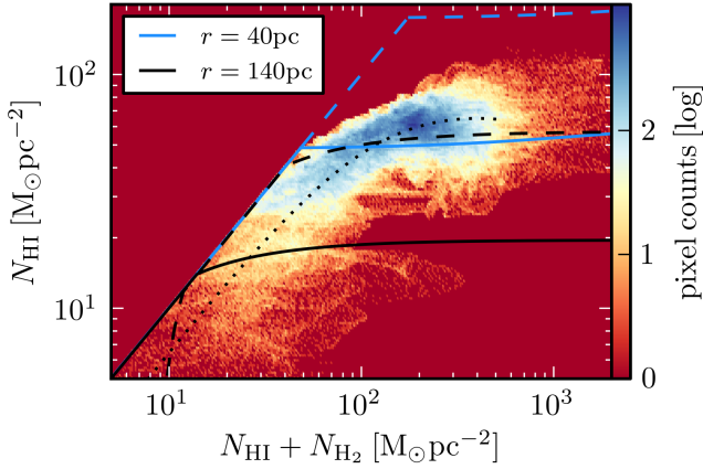
Fig. 17. Column density of the atomic hydrogen ( v_{\text{lsr}} = 60\text{--}120\text{ km s}^{-1} ) as a function of the total hydrogen column density ( N_{\text{HI}} + N_{\text{H}_2} ). The column density for the envelope ( r > 140\text{ pc} , N_{\text{HI}} = 107 \pm 20\text{ M}_\odot\text{ pc}^{-2} , N_{\text{H}_2} = 116 \pm 18\text{ M}_\odot\text{ pc}^{-2} ) is subtracted. The solid and dashed lines describe the theoretical model of Krumholz et al. (2008, 2009) for solar values ( G_0 = 1 , Z = 1 ) and for more realistic values of W43 ( G_0 = 5 , Z = 1.4 ), respectively. The blue and black colors represent the model parameters at different equivalent radii of r = 40 and 140\text{ pc} , respectively. The black dotted line shows the fitted curve of the elliptical annuli analysis introduced in Sect. 5.3.
