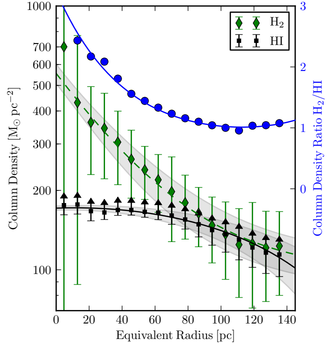
Fig. 13. Column density of HI and H 2 measured in elliptical annuli around W43 MM1. The x -axis presents the equivalent radius of these elliptical annuli. The black and green lines represent the fitted curves with the corresponding 1\sigma uncertainties shown as a gray shaded area. The larger symbols (diamonds for H 2 , squares for HI) present the averaged value of the elliptical annuli and their corresponding variations within the annuli. As the optical depth spectra saturates, we can only determine lower limits for the HI column density. The blue dots and line show the H 2 and HI column density ratio of the data and the fitted curves, respectively.
