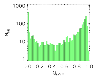
Fig. 23. Distribution of ANN-based estimation of Q_{good} , Q_{bad} , and Q_{ugly} for the MCXC catalogue. The vertical solid line shows the threshold Q_{bad} = 0.6 .
