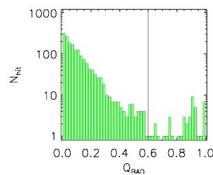
Fig. 23. Distribution of ANN-based estimation of Q_{good} , Q_{bad} , and Q_{ugly} for the MCXC catalogue. The vertical solid line shows the threshold Q_{bad} = 0.6 .
