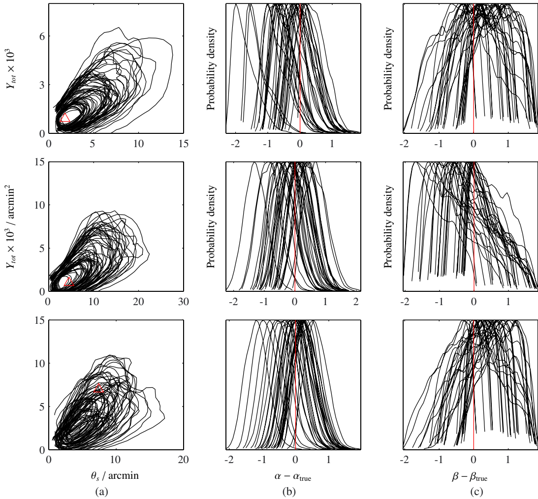
Fig. 29. Posterior distributions for simulated clusters with realistic noise levels (see text for details), and varying GNFW shape parameter values based on the REXCESS sample (Böhringer et al. 2007; Arnaud et al. 2010). a) shows the two-dimensional \theta_s and Y_{\text{tot}} posterior, and b) and c) show the one-dimensional posteriors for \alpha and \beta , shifted to be centred on the appropriate true value. In all cases \gamma is fixed to the universal value, \alpha has a truncated Gaussian prior based on the REXCESS sample, \beta is varied uniformly between 4.5 and 6.5, and the joint two-dimensional prior on Y_{\text{tot}} and \theta_s is used. Results for three different angular sizes are shown (from top to bottom, \theta_s = 1.8, 4.5 and 7.4 arcmin); the input parameter values are marked with red triangles and lines.
