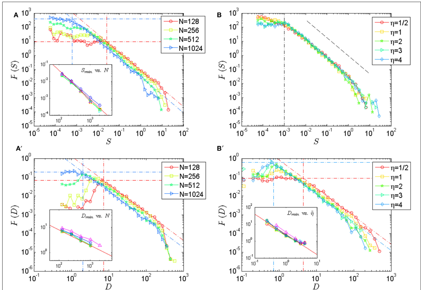
FIGURE 6 | Effect of the system size N and disorder strength \tilde{\eta} on the avalanche statistics. Main panel, top: Distribution of the avalanche size measured (A) for different N at constant c = 2 \times 10^{-5} , k = 10^{-2} and \tilde{\eta} = 1 , and (B) for different \tilde{\eta} at constant c = 2 \times 10^{-5} , k = 10^{-2} and N = 1024 . The axes are logarithmic. Main panel, bottom: Distribution of the avalanche duration measured (A') for different N at constant c = 2 \times 10^{-5} , k = 10^{-2} and \tilde{\eta} = 1 , and (B') for different \tilde{\eta} at constant c = 2 \times 10^{-5} , k = 10^{-2} and N = 1024 . All axes are logarithmic. In all panels, the power-law exponents \tau and \alpha are compatible with the universal values \tau = 1.28 and \alpha = 1.50 (inclined dashed line) predicted for c \rightarrow 0 and k \rightarrow 0 . Regarding the size, the lower cutoff S_{min} is
