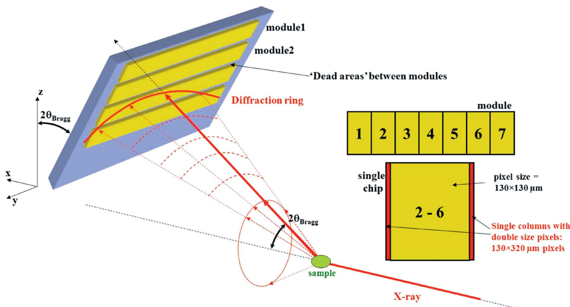
Figure 2 Schematic of the geometry of the XPAD (flat modules). The detector is carried by a motorized arm with two rotation angles ( \delta and \gamma , in the vertical and horizontal planes, respectively) used to adjust its angular position.
