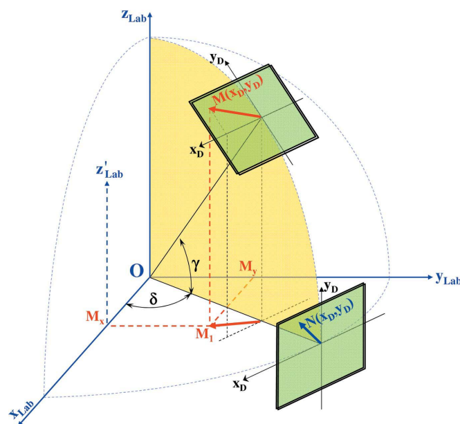
Figure 6 Positioning of the flat area detector. The X-ray incident beam is along the Ox_{\text{Lab}} axis. The situation described by He (2009) corresponds to the particular case of \gamma = 0^\circ . Angle M_xOM = 2\theta_{\text{Bragg}} is the Bragg diffraction angle and angle z'_{\text{Lab}}M_xM is the azimuth angle of the diffraction ring ( \theta_{\text{Bragg}} as illustrated in Fig. 1).
