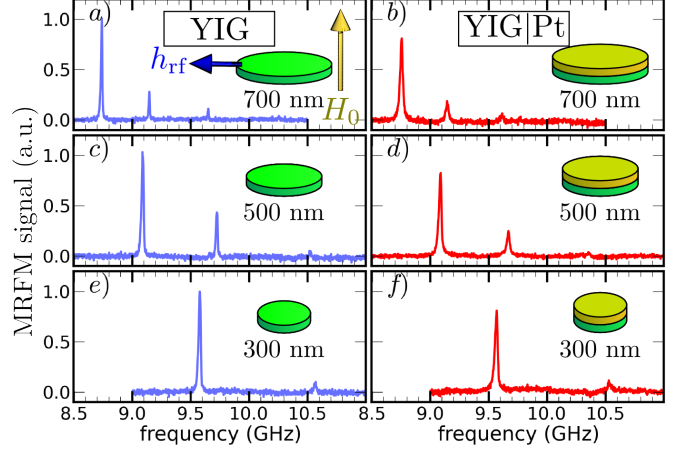
FIG. 2. Mechanical-FMR spectra at H_0 = 4.99 kOe of the 700, 500 and 300 nm diameter YIG disks arranged in rows by decreasing lateral size. The spectra of the pure YIG disks are shown in the left column (blue), while the ones covered with 13 nm of Pt are shown in the right column (red).
