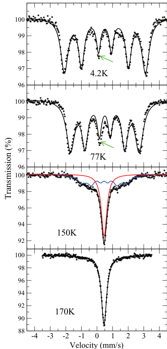
FIG. 3. (Color online) ^{57}\text{Fe} Mössbauer absorption spectra in ^{57}\text{Fe} -doped MnGe sample 1 at selected temperatures. At 4.2 and 77 K, the lines are fits to a standard six-line magnetic hyperfine pattern. At 150 K, the fit corresponds to a superposition of a single narrow line (in red) and of a six-line hyperfine pattern (in blue). At 170 K, the spectrum consists of a single narrow line.
