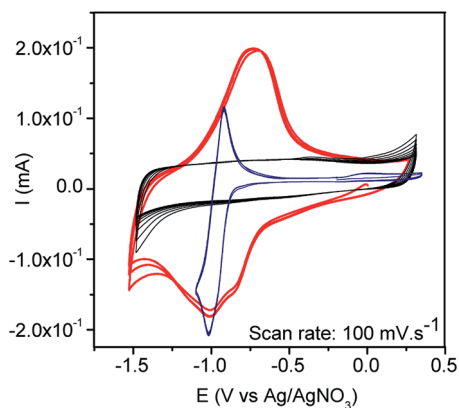
Fig. 3 Cyclic voltammetry for MWNTs (black line), glassy carbon with anthraquinone in solution (blue line), and MWNT/anthraquinone 2 (red line) in acetonitrile with 0.1 M LiClO 4 as the supporting electrolyte.
