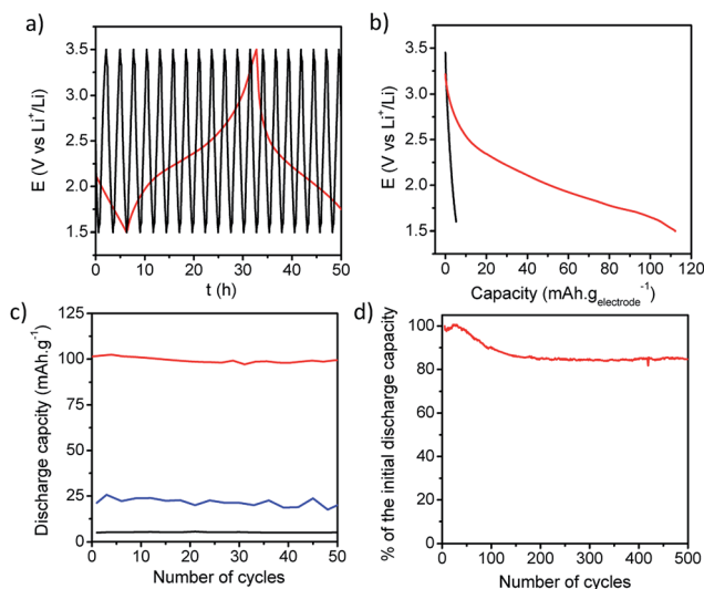
Fig. 4 (a) Charge/discharge profiles as a function of time for purified MWNTs (black) and MWNT/anthraquinone 2 (red) used as a positive electrode material in a Li/organic accumulator (2 mg samples, 5 \text{ mA g}_{\text{electrode}}^{-1} applied). (b) Discharge curves for purified MWNTs (black) and MWNT/anthraquinone 2 (red) as a function of the capacity. (c) Capacity retention of samples with purified MWNTs (black), MWNTs mixed with the anthraquinone molecule (blue) and MWNT/anthraquinone 2 (red) used as a positive electrode material. (d) Capacity retention over 500 cycles of a sample of MWNT/anthraquinone 2 used as a positive electrode material ( 50 \text{ mA g}_{\text{electrode}}^{-1} applied).
