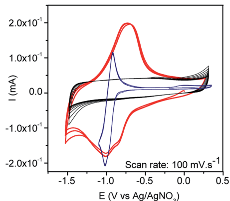
Fig. 3 Cyclic voltammetry for MWNTs (black line), glassy carbon with anthraquinone in solution (blue line), and MWNT/anthraquinone 2 (red line) in acetonitrile with 0.1 M \text{LiClO}_4 as the supporting electrolyte.
