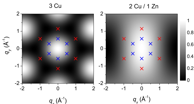
FIG. 9. (Color online) Intensity of the normalized form factor |A(q_x, q_y)|^2 related to sites 1 (left) and 2 (right), shown as grayscale maps. White (black) corresponds to a full (no) transmission. The site 3 does not show any filtering effect. Blue (red) crosses indicate the wave vectors of the cuboc2 ( q = 0 ) state.
