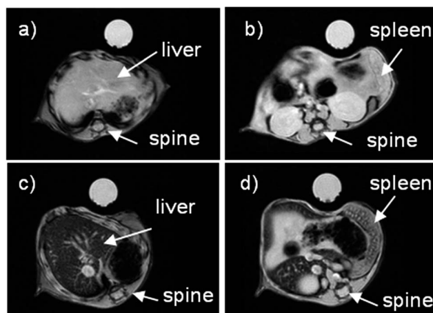
Fig. 4 T_2^* -weighted gradient echo ( \text{TE} = 5 \text{ ms} , \text{TR} = 300 \text{ ms} ) MR images of the mouse liver (left) and spleen (right). (a) and (b) Before injection; (c) and (d) at 30 min post-injection. The white circle corresponds to a tube filled with water serving as a MRI phantom.
