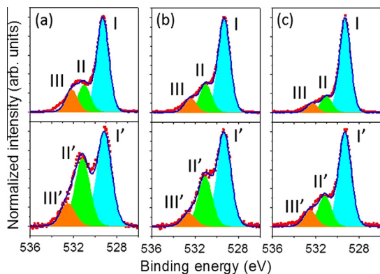
Figure 5. O 1s XPS core level spectra on BTO thin films grown with: (a) 250 W; (b) 400 W; (c) 550 W O 2 plasma power at normal (top) and 30° (bottom) take-off angle angles.
