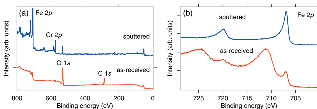
Fig. 1. Normalized XPS survey spectra (a) and Fe 2p (b) for 316L in the as-received state (red) and after in situ Ar + ion sputtering and 550 °C annealing (blue) in UHV. (For interpretation of the references to color in this legend, the reader is referred to the web version of the article.)
