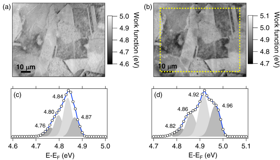
Fig. 3. Work function maps obtained from a pixel by pixel error function fit across the field of view for (a) Hg and (b) Al K \alpha excitation. The work function histograms extracted from the maps are shown in (c) and (d), respectively. The yellow dotted line in (b) indicates the effective FoV for the core level regions. (For interpretation of the references to color in this legend, the reader is referred to the web version of the article.)
