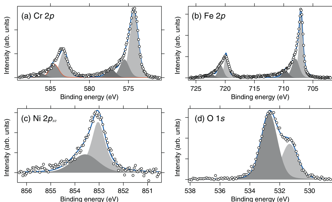
Fig. 5. Area averaged Cr, Fe 2p, Ni 2p 3/2 and O 1s core level spectra acquired using channeltron mode within a field of view of 115 \mu\text{m} corresponding to the SEM and PEEM images in Fig. 2, together with best least squares fits (see text for details). For clarity, only every second experimental point is shown in the Cr and Fe core level spectra.
