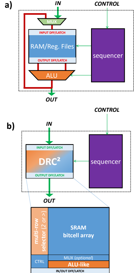
Figure 1 a) Conventional computing architecture vs. b) in-memory computing architecture. Moving into In-memory computing should allow speed increase, total area saving and less power consumption since physical distance between memory and computing unit is drastically reduced.
