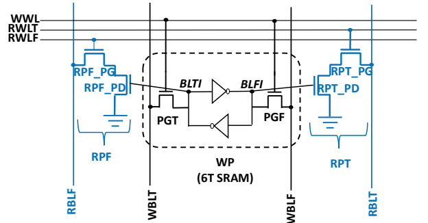
Figure 2 10-Transistors (10T) SRAM bitcell including one Write-Port (WP) and two Read-Port (RP), False (F) and True (T). Each RP is formed by its pass-gate (PG) and its pull-down (PD) transistors.
