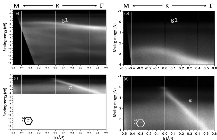
Figure 2. Angle-resolved photoemission spectroscopy spectra presenting the evolution of the electronic properties of the carbon-terminated 6H-SiC (0001) surface during the decoupling process. (a and b) The initial 6H-SiC(0001) 6\sqrt{3} \times 6\sqrt{3}R30^\circ buffer layer measured around K-point along the \Gamma -K-M direction; the white lines point out extrema of the g1 state modulation in k. (c and d) After several cycles of Si deposition and annealing, we obtain a totally decoupled one monolayer graphene.
