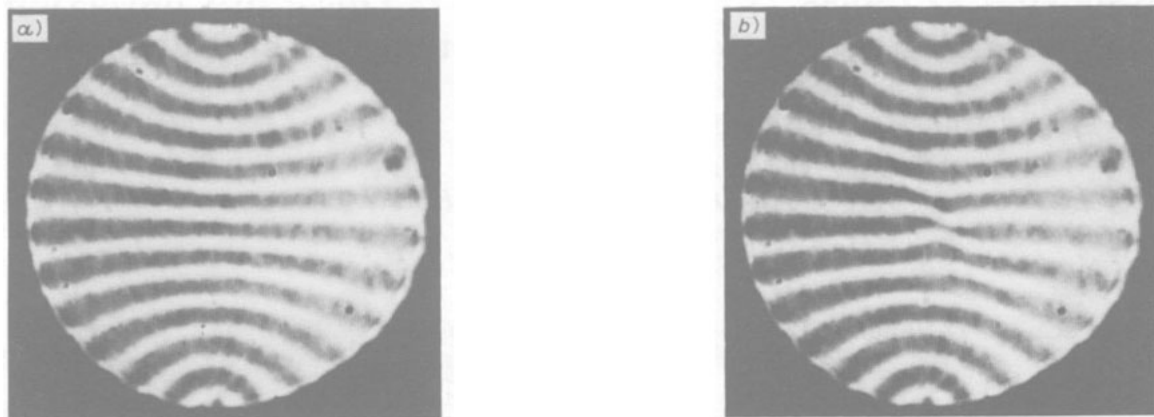
Fig. 1. – Pictures of the open container. a) Stationary pattern at \varepsilon = 0.55 . The y -axis is defined such that it joins the foci. b) Occurrence of the first instability at \varepsilon = 0.56 . Notice the skewed-varicose-like distortion.
