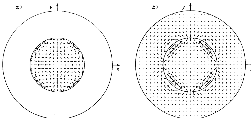
Fig. 2. – Mean-flow field solutions of the Cross-Newell equations. a ) The boundary of the convective domain (small circle) is nonpermeable to mean flows. Notice the back flows along the y -axis (the orientation is defined in fig. 1 a ). b ) The boundary of the convective domain is permeable to mean flows. The mean flow amplitude is then weaker than in the closed configuration. The shear at the boundary of the convective domain generates localized additional vertical vorticity, not represented on the picture.
