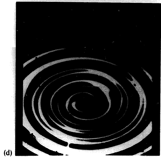
Fig. 2. Surface deformation at the vertical of a jet, for increasing values of the adimensional parameter \varepsilon = (F - F_c)/F_c . ( \phi = 1.44 mm; h = 10 mm): (a) \varepsilon = -0.2 ; (b) \varepsilon = -0.1 ; (c) \varepsilon = 0 : a transition is observed where the bump starts oscillating at a high eigenfrequency; (d) surface waves generated by the oscillatory motion of the bump. In both panels (c) and (d), stroboscopic lighting is used to visualize the phenomenon. In panels (a)–(c), the zoom magnification factor is 20.
