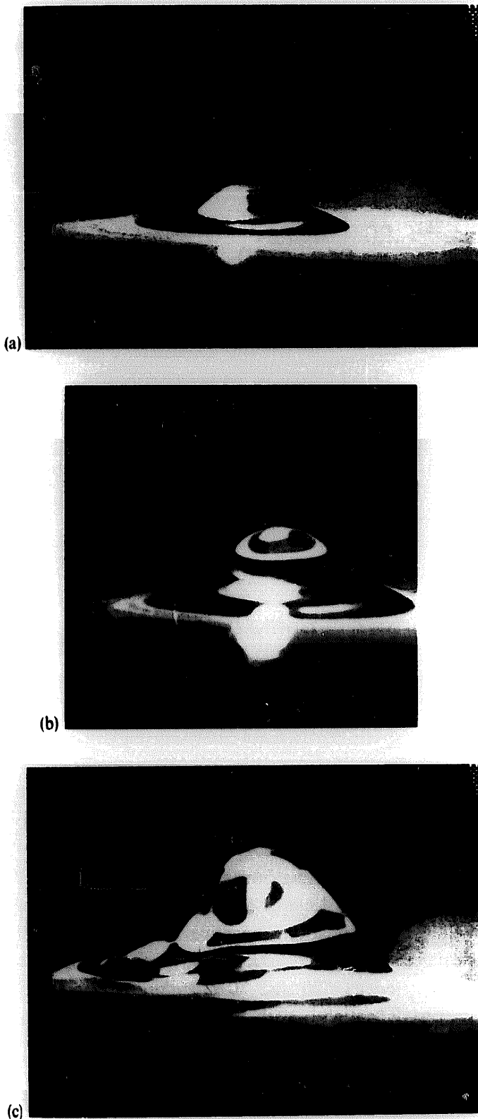
Fig. 2. Surface deformation at the vertical of a jet, for increasing values of the adimensional parameter \varepsilon = (F - F_c)/F_c . ( \phi = 1.44 mm; h = 10 mm): (a) \varepsilon = -0.2 ; (b) \varepsilon = -0.1 ; (c) \varepsilon = 0 : a transition is observed where the bump starts oscillating at a high eigenfrequency; (d) surface waves generated by the oscillatory motion of the bump. In both panels (c) and (d), stroboscopic lighting is used to visualize the phenomenon. In panels (a)–(c), the zoom magnification factor is 20.
