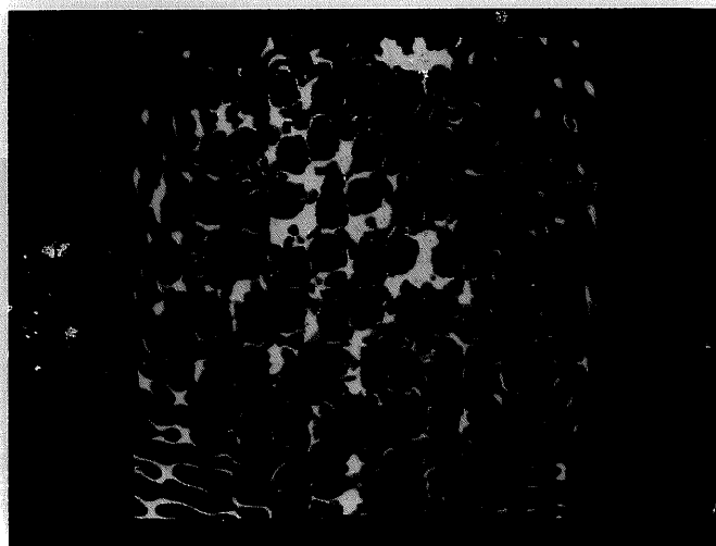
Fig. 7. Collective diagonal mode for a square geometry (seen from above).
