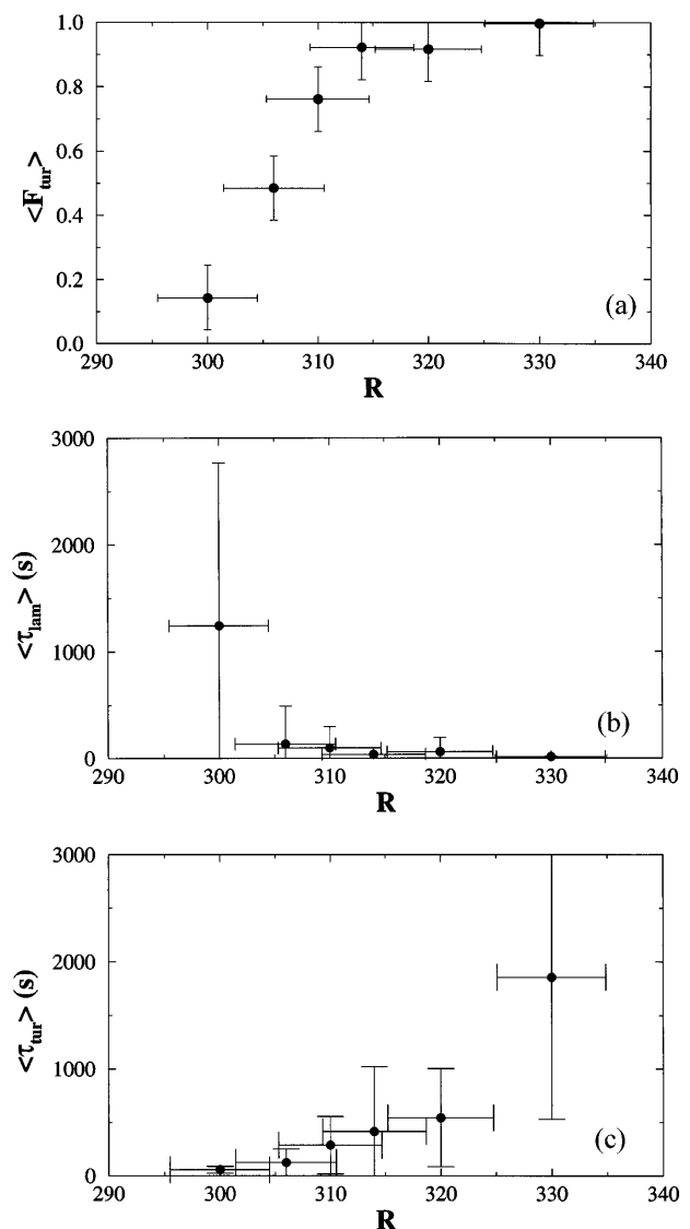
FIG. 5. Evolution of the turbulent fraction (a), the mean lifetime of laminar (b), and turbulent (c) events, with the Reynolds number.
