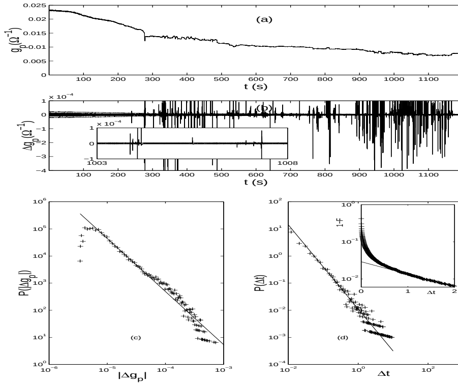
Fig. 2 – Analysis of \Delta g_p for a 33 \times 52 regular packing heated with the lamp. (a) Temporal evolution of the g_p . (b) Temporal evolution of \Delta g_p . Inset, expanded view on a few seconds scale (c) Log-log plot of the distribution P(|\Delta g_p|) . The straight line is a power law fit using Eq. 1 with \alpha_g = 1 . (d) Log-log plot of the probability density function P(\Delta t) . The straight line is a power law fit using Eq. 2, with \alpha_t = 0.61 . The inset shows the cumulative distribution which decays asymptotically as an exponential.
