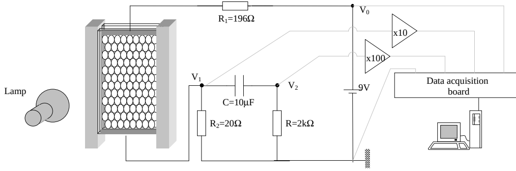
Fig. 1 – experimental set-up
