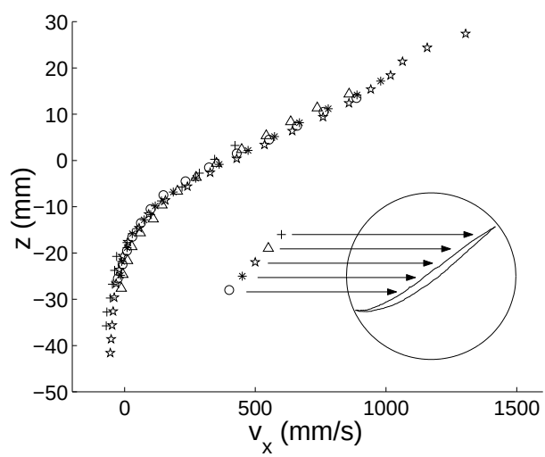
FIG. 6. Bonamy, Phys. Fluids
