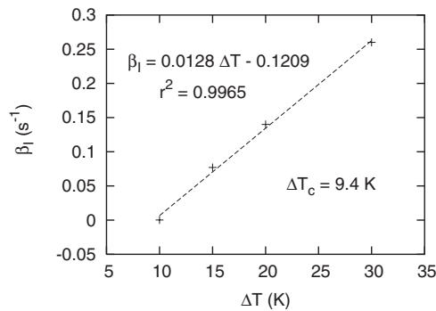
FIG. 10. Growing rate of the bidimensional instability ( \beta_I ) for different applied thermal difference \Delta T .
