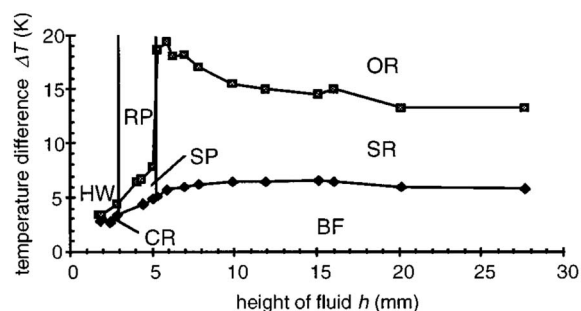
FIG. 1. Diagram of stability due to Favre [2] (see text for details).
