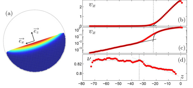
Fig. 1: (Colour on-line) (a)–(c) time and ensemble averaged streamwise velocity v_x for a \Omega = 6 rpm rotation velocity: (a) map with normalized colormap, (b) with linear and (c) logarithmic z -axis as a function of the depth z at the center of the drum ( x=0 ). (d) Volume fraction \nu as a function of the depth z at the center of the drum ( x=0 ). Velocities are non-dimensionalized by \sqrt{gd} , where g is the gravity constant and d the mean bead diameter. In (b) and (c), solid lines are the result of a linear and an exponential data fit.
