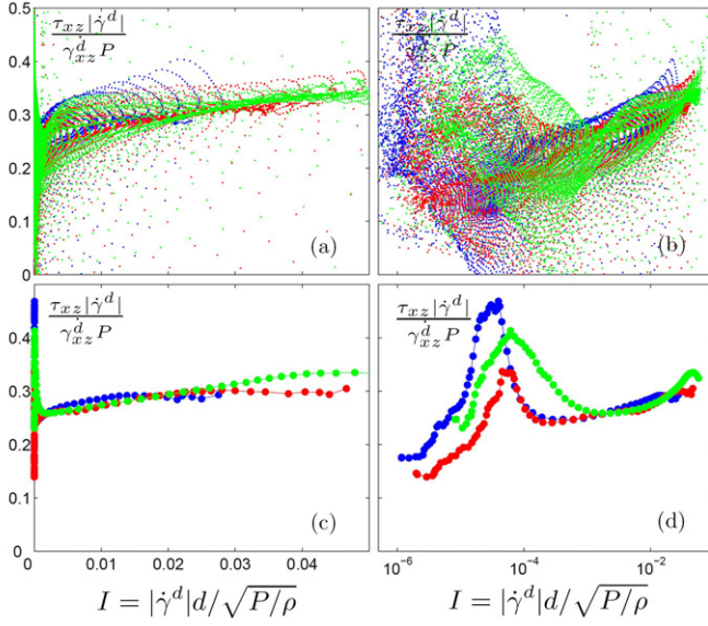
Fig. 2: (Colour on-line) Effective friction coefficient \tau_{xz}|\dot{\gamma}^d|/\gamma_{xz}^d P as a function of the inertial number for time and ensemble averaged data, (a) and (b) over the whole 2D drum, (c) and (d) at the center of the drum ( x = 0 ), with linear, (a) and (c), and logarithmic, (b) and (d), x -axis. Green/light gray points correspond to \Omega = 12 rpm, red/intermediate gray points to \Omega = 6 rpm, and blue/dark gray points to \Omega = 2 rpm.
