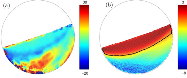
Fig. 6: (Colour on-line) (a) Map of the angle difference between principal directions of \tau_{ij} and \dot{\gamma}_{ij}^d for \Omega = 12 rpm. (b) Map of the logarithm of the norm of the strain rate tensor times the half drum rotation duration \log|\dot{\gamma}^d|/2\Omega for \Omega = 12 rpm. We indicate with a black line the limit where this deformation \delta \equiv |\dot{\gamma}^d|/2\Omega = 1 .
