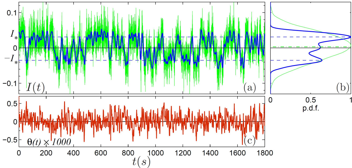
Figure 8. (a) Global angular momentum I(t) for an experiment performed at Re = 39000 for \theta = \overline{\theta(t)} = 0 . The green thin line is SPIV data I(t) sampled at 15 Hz and the blue thick line corresponds to 0.15 Hz low-pass filtered data I_f(t) . (b) Probability density functions (PDF) with the same color code. Blue dashed lines indicate the two most-probable values \pm I_* of I_f(t) and green dash-dot lines indicate the mean value \bar{I} . (c) Time-series of \theta(t) as produced by the motor regulation in unit of 10^{-3} : the correlation with I(t) is negligible (see text).
