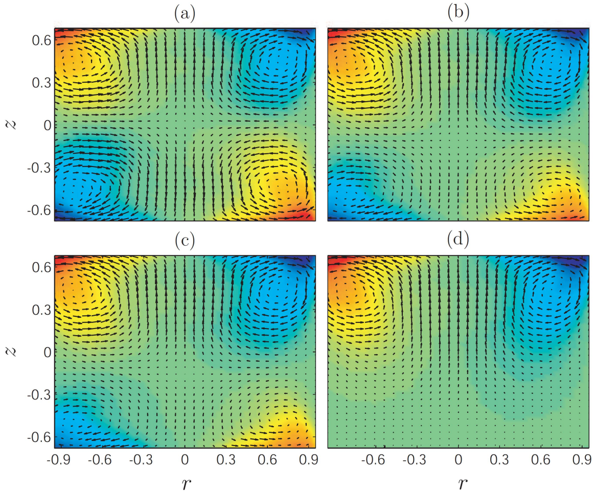
Figure 2. Maps of velocity fields in the meridional plane (r, z) —the rotation axis is vertical at r = 0 and the r \leftrightarrow -r symmetry of the maps reveals the flow axisymmetry— for the laminar ( Re = 120 \pm 25 ) von Kármán flow for different values of the symmetry control parameter \theta : (a) \theta = 0 , (b) \theta = -0.11 , (c) \theta = -0.19 , (d) \theta = -1 . The color maps, from blue to red (“jet” colormap), the azimuthal velocity u_\varphi , whereas the arrows map the (u_r, u_z) field. The resolution of the fields has been reduced by a factor 2 for better visibility. Positions r and z are given in units of vessel radius R .
