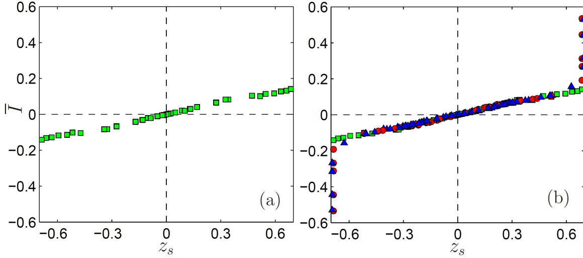
Figure 4. Experimental observation of proportionality between time-averaged global angular momentum \bar{I} and mean shear layer altitude z_s for (a) laminar flow Re = 120 \pm 25 (green squares, \bar{I}/z_s = 0.235 \pm 0.005 ) and (b) turbulent flows at Re = 67\,000 (red circles, \bar{I}/z_s = 0.227 \pm 0.005 ) and Re = 890\,000 (blue triangles, \bar{I}/z_s = 0.23 \pm 0.01 ). Each data series is obtained through plotting \bar{I}(\theta, Re) as a function of z_s(\theta, Re) for varying \theta and constant Re . At high Re , this proportionality holds for -0.1 \lesssim \theta \lesssim 0.1 , i.e. while the shear layer position z_s is not saturated to the impellers positions \pm 0.7 R .
