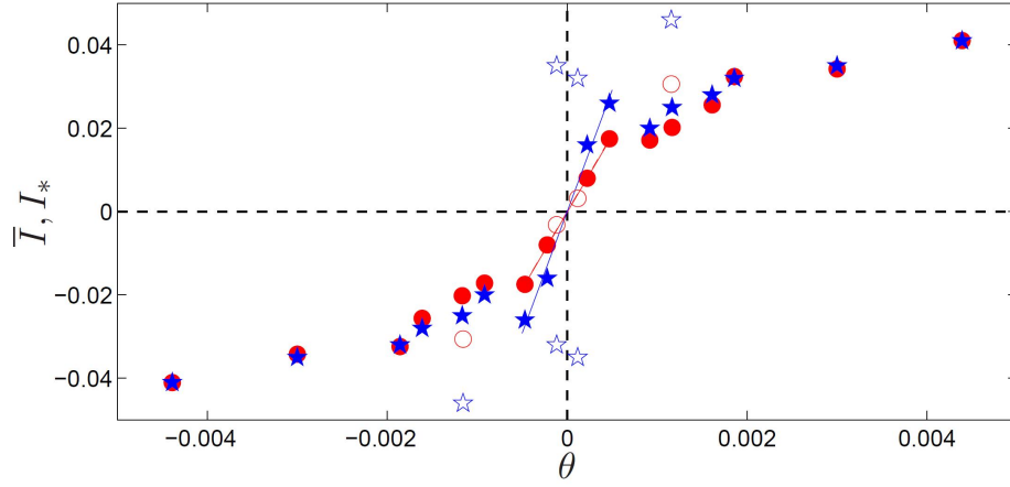
Figure 9. Mean \bar{I} (red circles) and most-probable I_* (blue stars) values of the global angular momentum I(t) for Re \sim 40\,000 . Close symbols come from a set of moderate-resolution data at Re = 37\,000 \pm 2\,000 ( f = 12\text{Hz} , 1 200 SPIV fields acquired at 1.7Hz), whereas open symbols come from high-resolution time-series at Re = 41\,000 \pm 2\,000 ( f = 8\text{Hz} , 9 000 or 27 000 SPIV fields acquired at 15Hz as, e.g., in figure 8) acquired in a different glycerol-water mixture. The data have been symmetrized with respect to \theta = 0 and, for the data point at \theta \simeq 0 of the second series, we plot the two most-probable values \sim \pm I_* corresponding to the two peaks of the PDFs as in figure 8(b).
