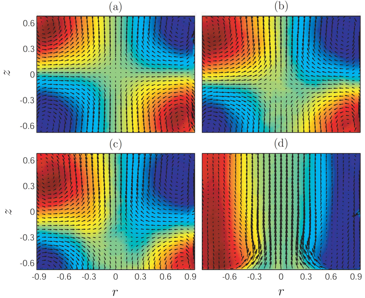
Figure 6. Maps of mean velocity fields of the turbulent von Kármán flow at Re = 890\,000 for different values of \theta : (a) \theta = 0 , (b) \theta = -0.0036 , (c) \theta = -0.0147 , (d) \theta = -1 , with same layout as figure 2. The r \leftrightarrow -r symmetry of the maps reveals that the time-averaged mean fields are axisymmetric.
