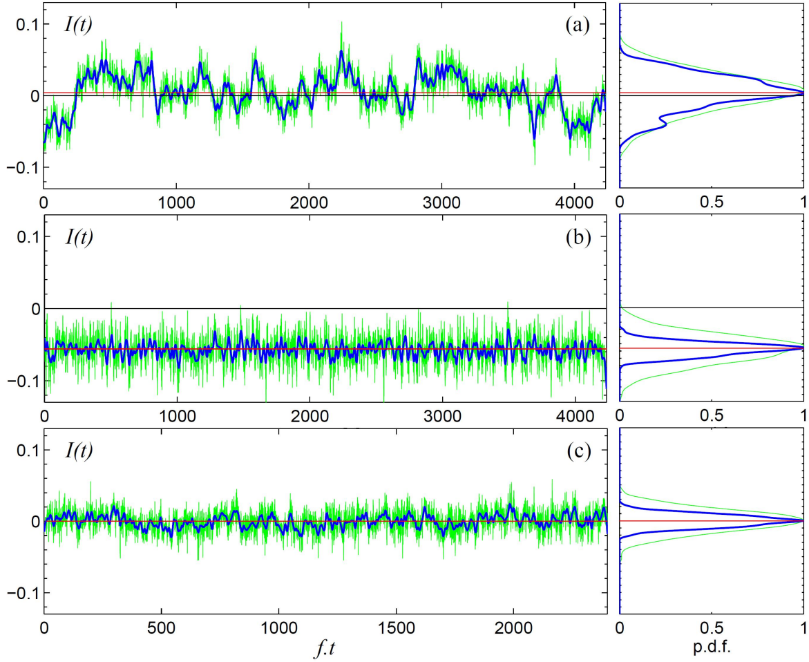
Figure 3. Global angular momentum I(t) as a function of non-dimensional time f.t for experiments performed at Re = 126\,700 \pm 200 with (a) \theta = 0 \pm 10^{-4} and (b) \theta = -0.0084 and (c) at Re = 890\,000 and \theta = 0 . Green thin signals are SPIV data I(t) sampled at 15 Hz and blue thick signals correspond to low-pass filtered data I_f(t) . Corresponding right figures shows the probability density functions (PDF) of the signals with same color code. The red lines indicate the most-probable values of I_f(t) .
