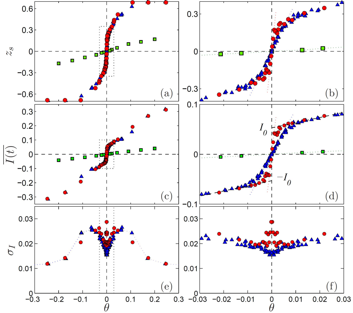
Figure 7. Turbulent regimes at Re = 67\,000 \pm 2\,000 (red circles) and Re = 890\,000 \pm 140\,000 (blue triangles): axial position of the stagnation point z_s (a-b) and global angular momentum I —mean \overline{I(t)} (c-d) and standard error \sigma_I (e-f)—as a function of \theta . Wide span -0.3 < \theta < 0.3 on the left side (a,c,e) and \times 10 zoom -0.03 < \theta < 0.03 on the right side (b,d,f). Data for the laminar regime at Re = 120 (green squares) from figure 5 are also plotted for comparison. The data have been symmetrized with respect to \theta = 0 . Dashed lines in (d) indicates the tilted plateaus independent of Re and their extrapolations to \pm I_0 .
