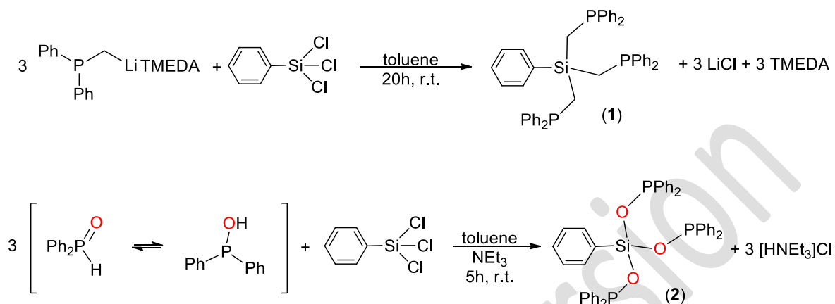
Scheme 1: Synthesis of the \text{PhSi(XPPH}_2)_3 ligands ( \text{X} = \text{O}, \text{CH}_2 ).
