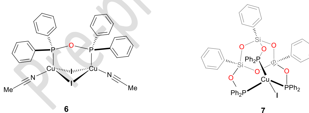
Scheme 3: Complexes 6 and 7 obtained from degradation of ligand 2
