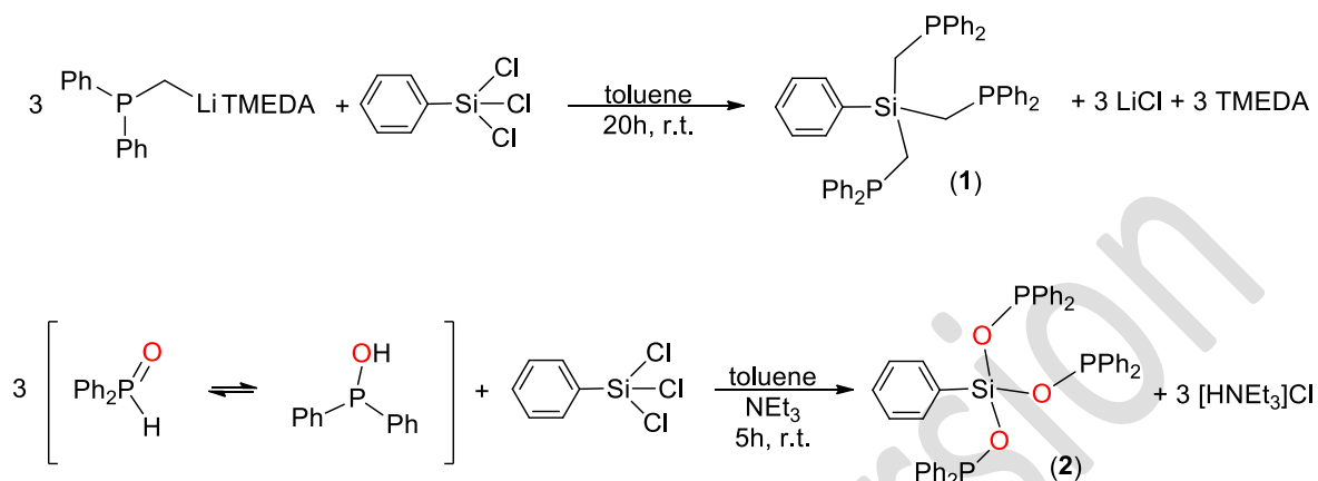
Scheme 1: Synthesis of the \text{PhSi(XPPH}_2)_3 ligands ( \text{X} = \text{O, CH}_2 ).
