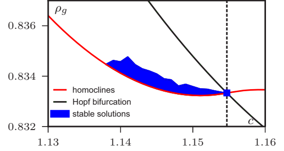
FIG. 14. (Color online) The blue region is the subset of admissible propagative solutions which are linearly stable. None of the solutions for c > c^* is stable in the hydrodynamic equations. v_0 = \lambda = \xi = a_4 = \varphi_g = 1 . We use system sizes L_x = 300 or more (adapted to fit the solution) with resolution dx = 0.5 and dt = 0.1 .
