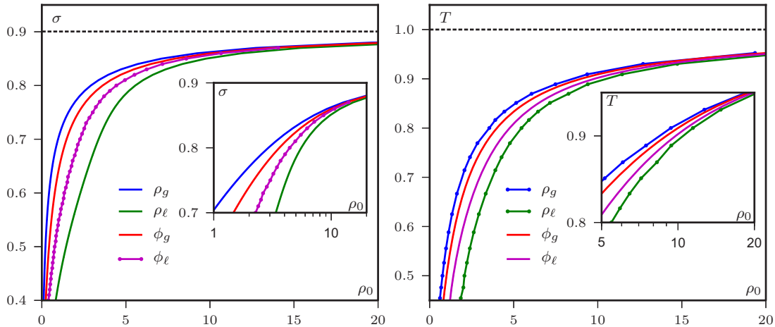
FIG. 17. (Color online) Phase diagram of the Vicsek (left) and Ising (right) hydrodynamic equations. The spinodal lines \varphi_g and \varphi_\ell are known exactly except \varphi_\ell in the Vicsek hydrodynamic equation which we computed numerically by looking at the stability of systems of size 50 \times 50 . The binodals \rho_g and \rho_\ell are the coexisting densities of phase-separated (heteroclinic) solutions as explained in the text. The dashed line indicates the asymptote above which only disordered solutions exist. Insets are close-ups on the high-density regions with a logarithmic scale on the x axis. Parameters: v_0 = D = 1 = r = 1 (Ising), v_0 = 1 (Vicsek).
