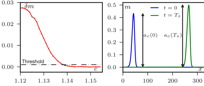
FIG. 13. (Color online) Stability of homoclinic orbits in the hydrodynamic equations. \Delta c is the difference in the amplitude of the solution measured between t = 0 and t = T_s . The solution is declared to be linearly stable if \delta m(T_s) , defined in Eq. (53) is smaller than a threshold that we take at 10^{-3} . v_0 = \lambda = \xi = a_4 = \varphi_g = 1 , c = 1.125 (right).
