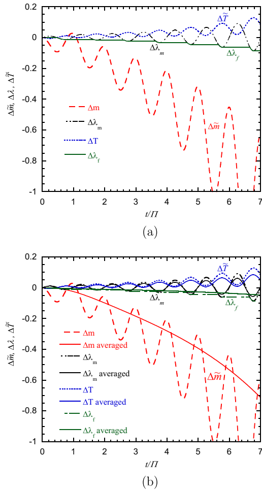
Fig. 4. Temporal evolution of system variables. The parameters \gamma = 1.36 , \theta = 160 , \mu/\psi = 6.4 , \sigma = 0.1 , \Omega = 800 , \xi = 100 , \zeta = 700 , \phi = 10^3 , and f = 3.2 \times 10^{-4} used hereafter are close to those of oxygen at 70 K [11]. Other parameters are the same as for Fig. 2. The gas mass variation is rescaled: \Delta\tilde{m} = \Delta m/m_2 . (a) Evolution accounting for the temporal temperature variation in the tube and in the liquid. (b) Comparison between the solution of the PWL set (51) and its averaging approximation (B.4) for the imposed temperature distribution.
