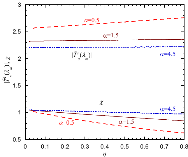
Fig. 9. The critical temperature gradient and the corresponding to it reduced meniscus position \chi for the imposed T_s model as functions of \eta for different evaporator lengths \alpha and \varepsilon = 0.05 . The other parameters are those of Fig. 8.
