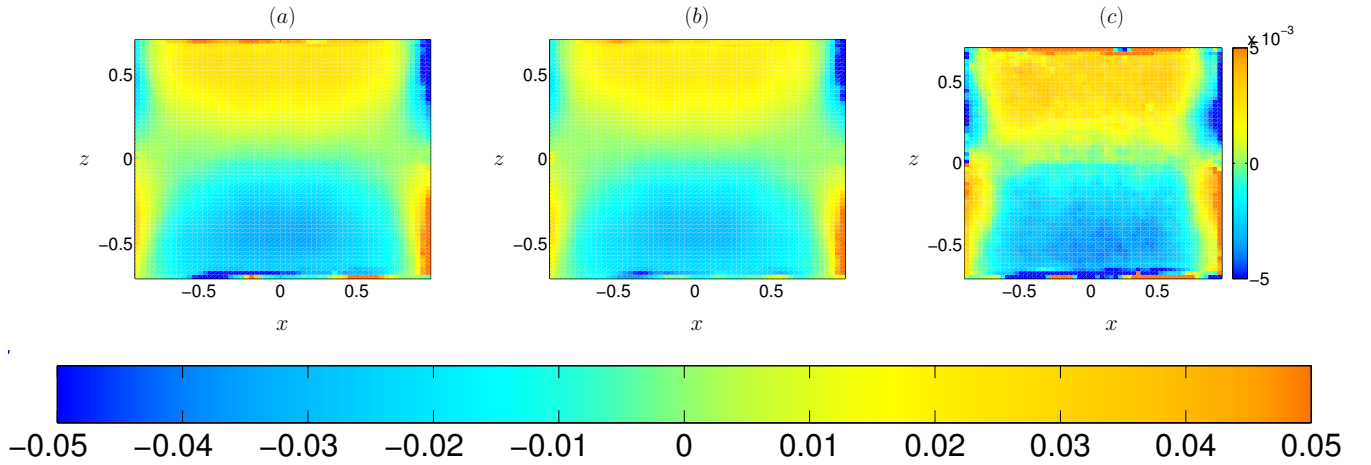
FIG. 7: Typical maps of \overline{J^z} : a) mean energy transfer through the system, b) contribution of the mean flow, c) contribution of the fluctuations
