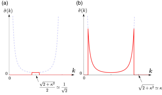
FIG. 13. (Color online) Reduced growth rate of b waves as a function of wave number k , for a waves at wave number \kappa . The dashed curve is (\sqrt{2 + \kappa^2} - k)^{-2} + k^{-2} . Left-hand panel: for \kappa \ll 1 , b waves grow at wave number k \simeq 1/\sqrt{2} . Right-hand panel: for \kappa \gg 1 , the growth rate has two strong maxima, one at k \simeq 1/\kappa and one at k \simeq \kappa .
