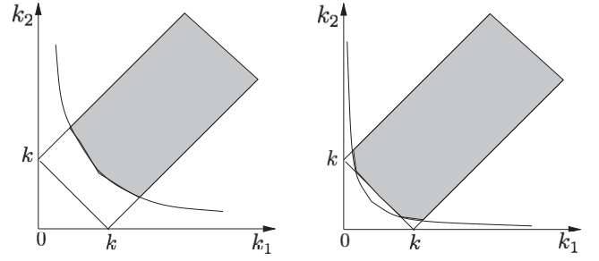
FIG. 5. Integration domain \mathcal{D}_a(k) for k < 1/\sqrt{2} (left-hand panel) and k > 1/\sqrt{2} (right-hand panel).
