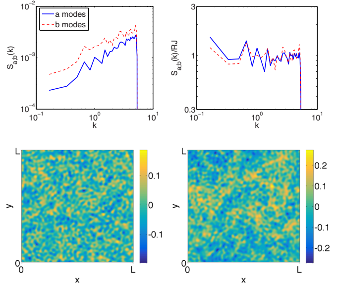
FIG. 8. (Color online) \alpha = -0.5 : in the stationary state, \mathcal{F} = 2.42 \in (K/3, K/2) , so we expect a Rayleigh-Jeans distribution. Top: spectra of a and b modes (left), and spectra normalized by a Rayleigh-Jeans spectra with \mu = 1.67 and T = 7 \times 10^{-4} (right). Bottom: snapshots at final time of the \lambda and \chi fields.
