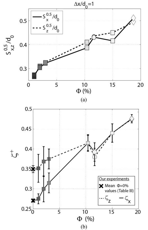
FIG. 8. (a) Normalized roughness amplitudes in the x and z directions \sqrt{S(d_0)}/d_0 versus porosity \Phi . (b) Large-scale roughness exponents \zeta^+ vs \Phi . Symbols match the experiments in Fig. 7. Crosses correspond to the averaged exponent values in Table III.
