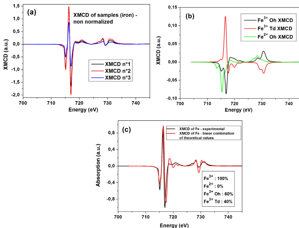
Fig. 2. Experimental XMCD spectra at the L_{2,3} edge of Fe in the samples (a); theoretical XMCD plots of \text{Fe}^{3+} Oh , \text{Fe}^{3+} Td and \text{Fe}^{2+} Oh (b); from Ref. [19], fitted XMCD spectra of the sample 2 recorded at the L_{2,3} edge of Fe, obtained by the least-squared combinatory method (c).
