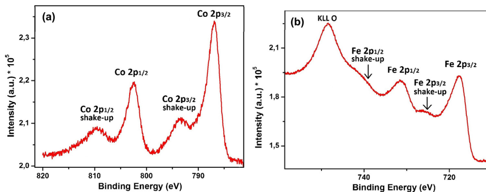
Fig. 3. XPS spectrum of Co in \text{CoFe}_2\text{O}_4 for sample 3 (a). XPS spectrum of Fe in \text{CoFe}_2\text{O}_4 for sample 3 (b).
