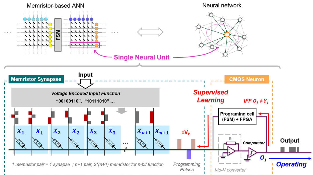
Figure 1. Schematic representation of the neuromorphic learning system.
