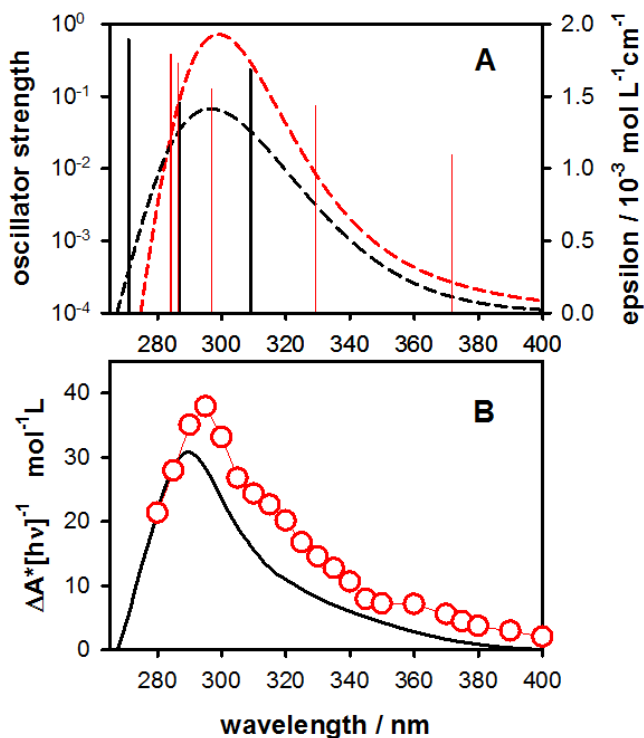
Figure 3. (A) Low energy electronic transitions of A=A and AA* dimers (black) and the precursor \phi\text{I} (red); PCM/TD-CAM-B3LYP/6-31+G(d,p)//PCM/M052X/6-31G(d) calculations. The energies have been homogenously decreased by 0.45 eV, which is the difference between the experimental absorption maximum of adenine and the vertical absorption energy computed at the adopted level of theory. In dashes: calculated differential absorption spectra corresponding to the disappearance of reacting adenines and the formation of \phi\text{I} (red) and A=A and AA* (black, assuming that their yields are roughly equal, in line with literature 6 ); the oscillator strength is proportional to the spectral area; the spectral width is 0.4 eV. (B) Spectrum obtained for (dA) 20 at 20 ms (red) compared to the difference of steady-state absorption spectra recorded after and before irradiation (black). The spectra are normalized by the concentration of absorbed photons [hv].
