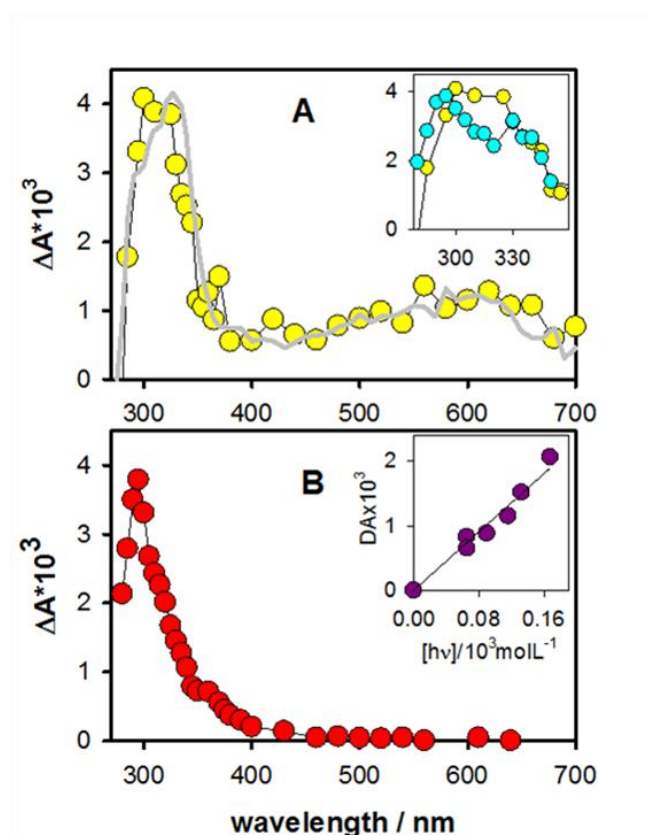
Figure 4. Time-resolved absorption spectra (circles) obtained for (dA) 20 at 1.7 \mu s (A) and 20 ms (B) following laser excitation at 266 nm. The grey line in A corresponds to the spectrum of the adenine radical (from reference 18 ; in arbitrary units). Inset in A: normalized spectra obtained for different ratios of ejected electron versus absorbed photons; 1.5 \times 10^{-3} (yellow) and 0.3 \times 10^{-3} (cyan). Inset in B: dependence of the transient absorbance at 340 nm and 20ms on the concentration of absorbed photons.
