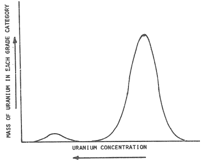
Fig. 5. Bimodal relationship between cumulated uranium resources and ore grades [9].
