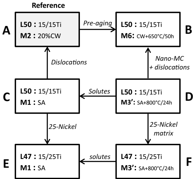
Fig. 3. Schematics of the sample names and the associated thermomechanical treatments. Arrows indicate the investigated effects.
