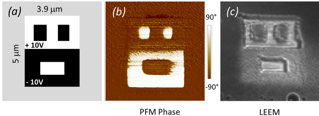
FIG. 2. (a) Pattern written by PFM on a 15 nm BaTiO 3 /Nb: SrTiO 3 (001). (b) PFM phase image after writing and (c) LEEM image of the same region for incident electron energy of 1.4 eV.
