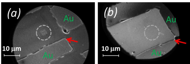
FIG. 3. LEEM image for an incident electron energy of 1.4 eV on a 15 nm BaTiO 3 /Nb: SrTiO 3 (001) sample at the same region as in Fig. 2 (a) after PFM poling, (b) after PFM poling and +8 V EC poling. Gold landmarks are shown and red arrows and grey circles indicate the same place for the two images.
