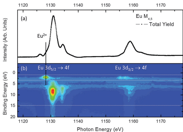
Fig. 3 (a) Near band edge X-ray absorption spectrum for the mixed valence \text{EuCl}_{2.85} salt deposited on the Au(111) reconstructed surface measured in the photon energy range of Eu 3d–4f ( M_{4,5} absorption edge) in TEY mode. (b) Resonant photoemission map of the photon energy (1118–1178 eV) corresponding to 3d \rightarrow 4f absorption edges. The right part corresponds to 3d_{3/2} \rightarrow 4f transitions. The left part is related to 3d_{5/2} \rightarrow 4f transitions, dash lines delimit the area of localized resonant states.
