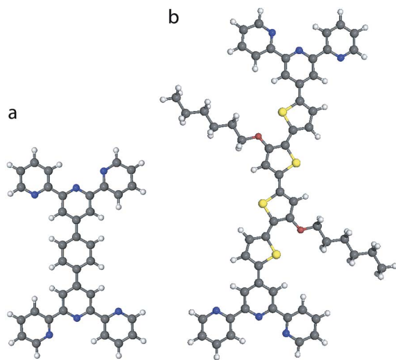
Fig. 2 Schematic representation of (a) 4',4'''-(1,4-phenylene) bis(2,2':6',2''-terpyridine) ( C_{36}H_{24}N_6 ) and (b) 4'-(3',4''-dihexyloxy-5,2':5',2'''-quaterthien-2,5'''-diyl)-bis(2,2':6',2''-terpyridine) (4T-bisterpy) molecule ( C_{58}H_{52}N_6O_2S_4 ). Carbon atoms are gray, oxygen atoms are red, nitrogen atoms are blue, hydrogen atoms are white, and sulfur atoms are yellow respectively.
