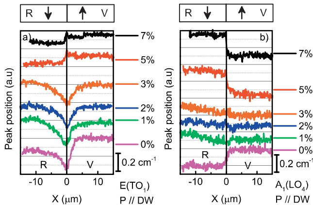
Figure 2 Peak position of (a) E(TO_1) and (b) A_1(LO_4) for line-scan from reversed (R) to virgin (V) domains for different amounts of magnesium before annealing. The data are vertically shifted for clarity and the scale bar gives the amplitude of the frequency shift.
