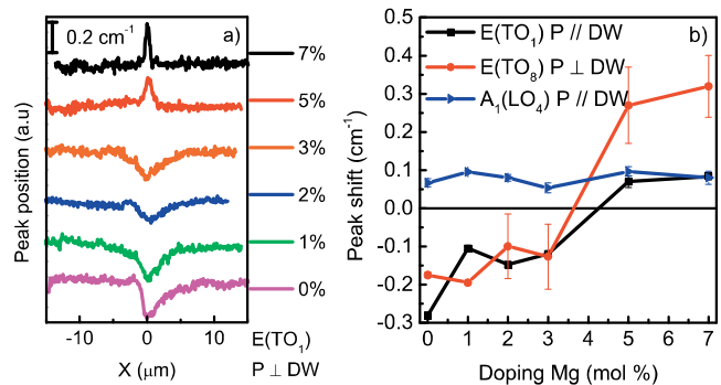
Figure 3 (a) Peak position of E(TO_1) across a domain wall after annealing. (b) Peak shifts at the domain wall. Error bars represent the standard deviation calculated from measurements on three different domain walls.
